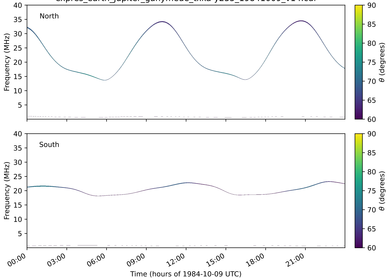
expres_earth_jupiter_ganymede_txka-y235_19841009_v14.cdf
