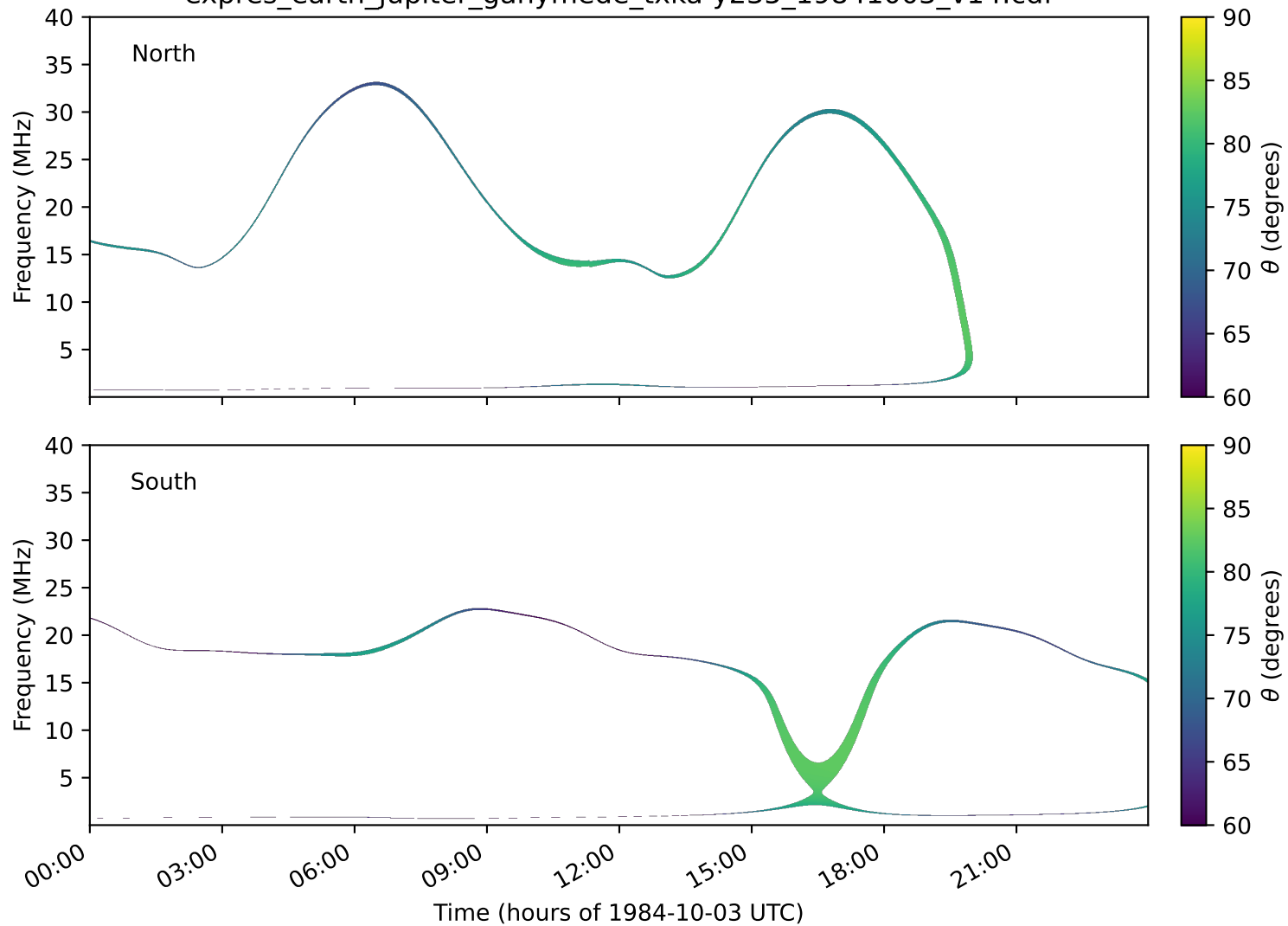
expres_earth_jupiter_ganymede_txka-y235_19841003_v14.cdf
