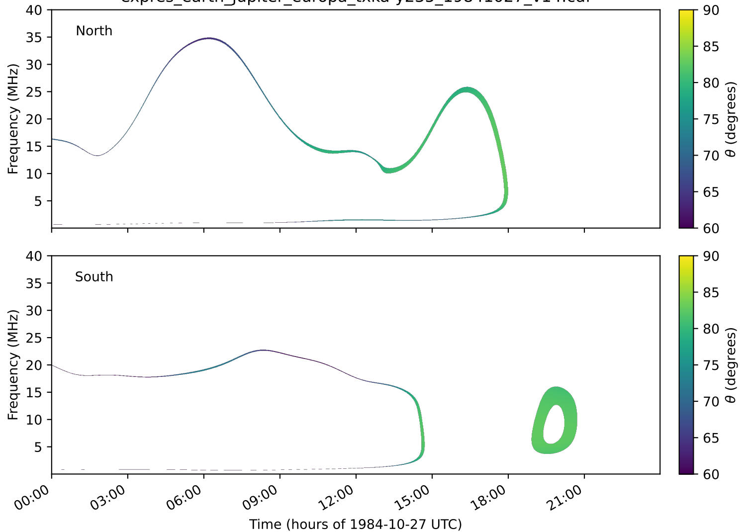
expres_earth_jupiter_europa_txka-y235_19841027_v14.cdf
