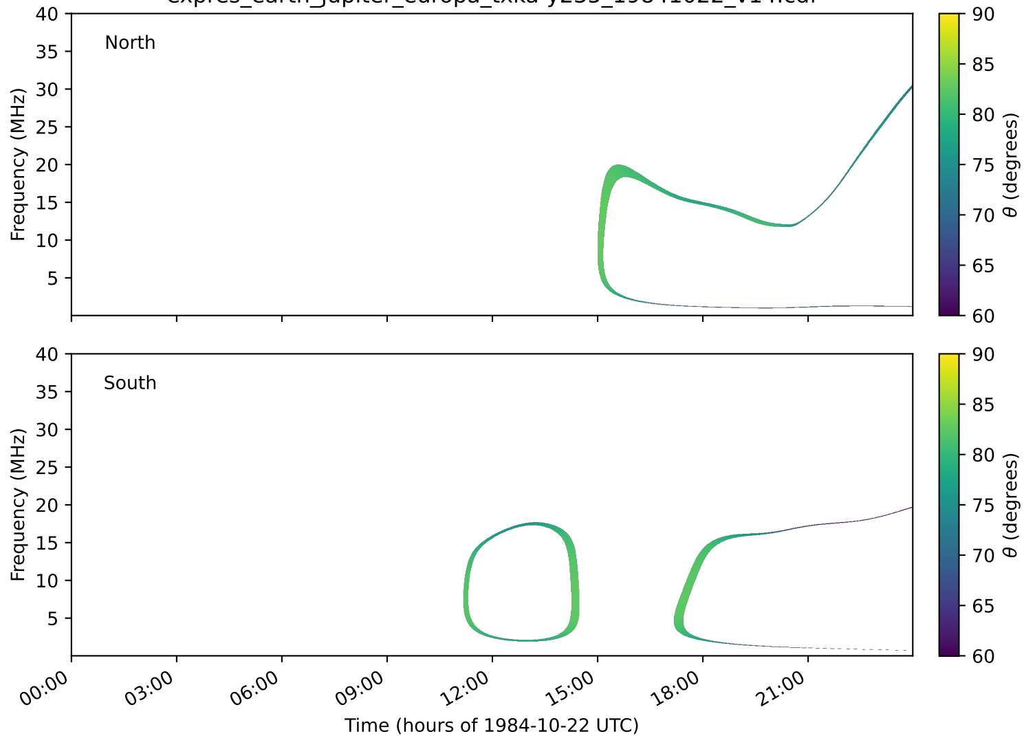
expres_earth_jupiter_europa_txka-y235_19841022_v14.cdf
