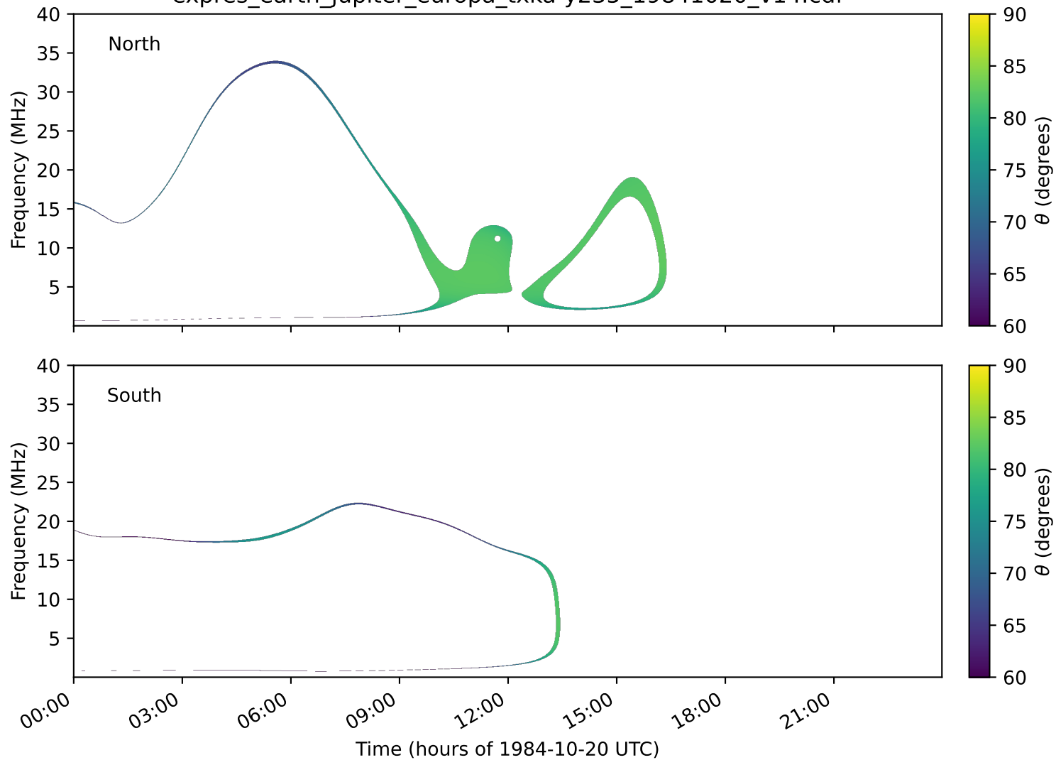
expres_earth_jupiter_europa_txka-y235_19841020_v14.cdf
