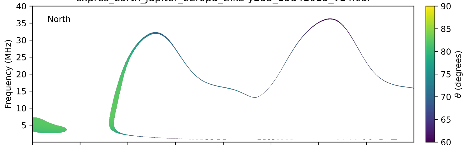
expres_earth_jupiter_europa_txka-y235_19841019_v14.cdf
