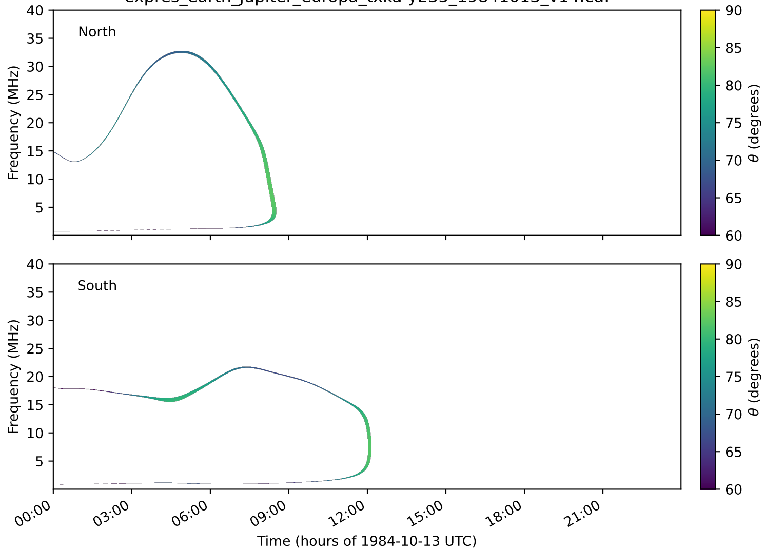
expres_earth_jupiter_europa_txka-y235_19841013_v14.cdf
