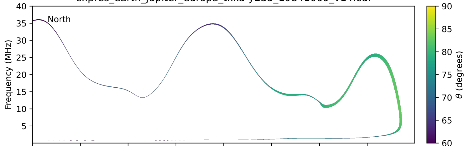
expres_earth_jupiter_europa_txka-y235_19841009_v14.cdf
