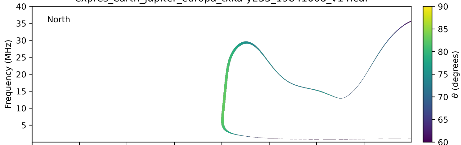
expres_earth_jupiter_europa_txka-y235_19841008_v14.cdf
