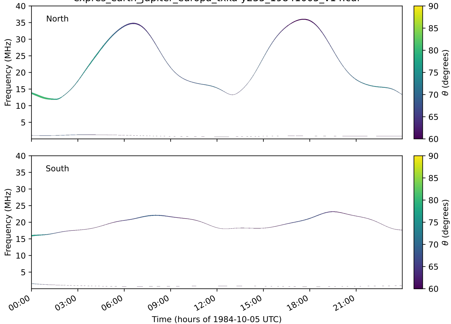
expres_earth_jupiter_europa_txka-y235_19841005_v14.cdf
