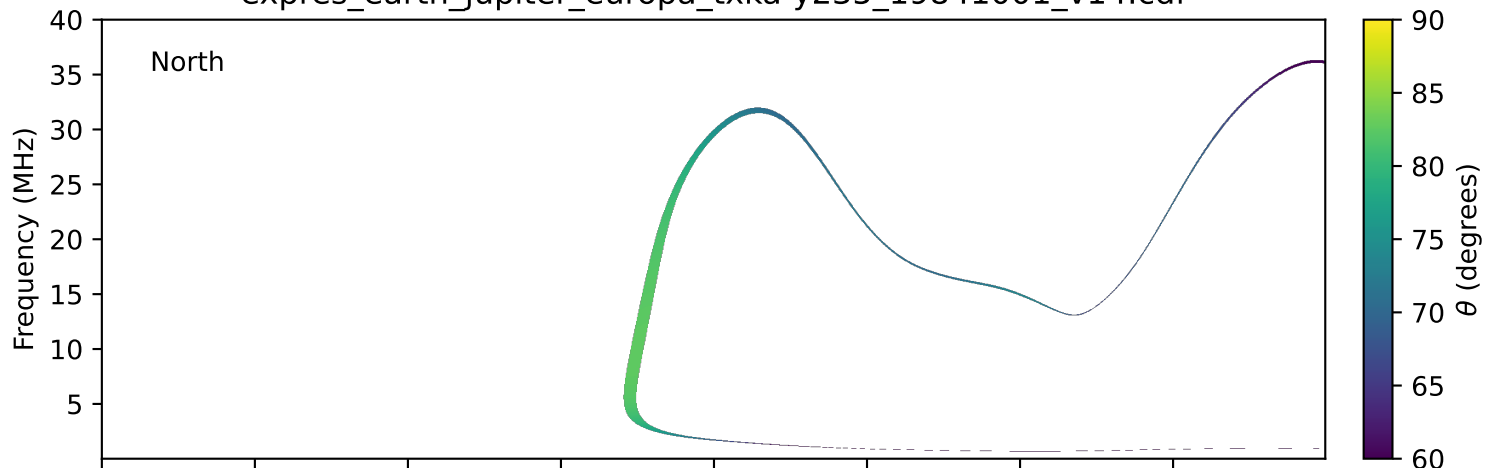
expres_earth_jupiter_europa_txka-y235_19841001_v14.cdf
