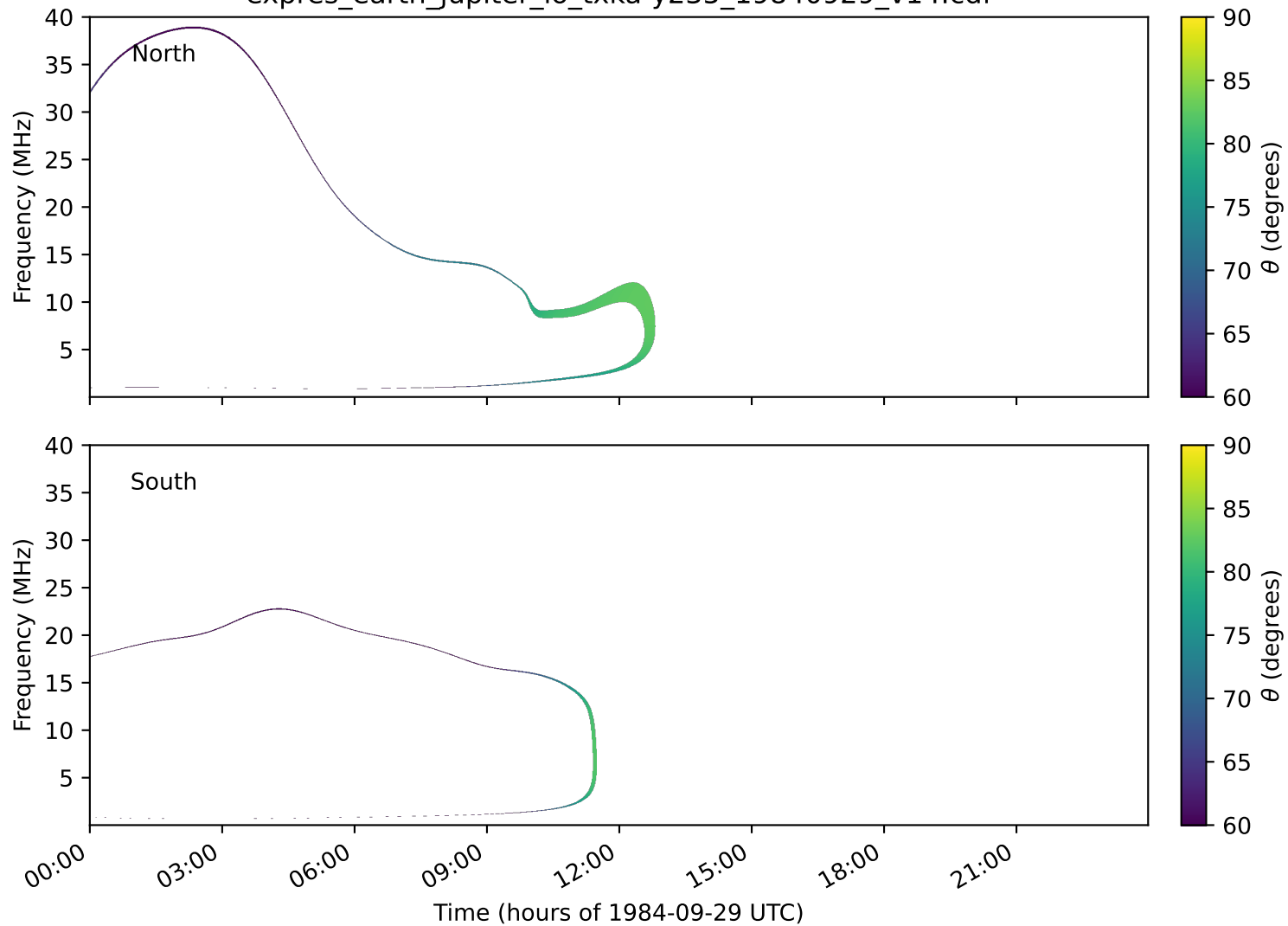
expres_earth_jupiter_io_txka-y235_19840929_v14.cdf
