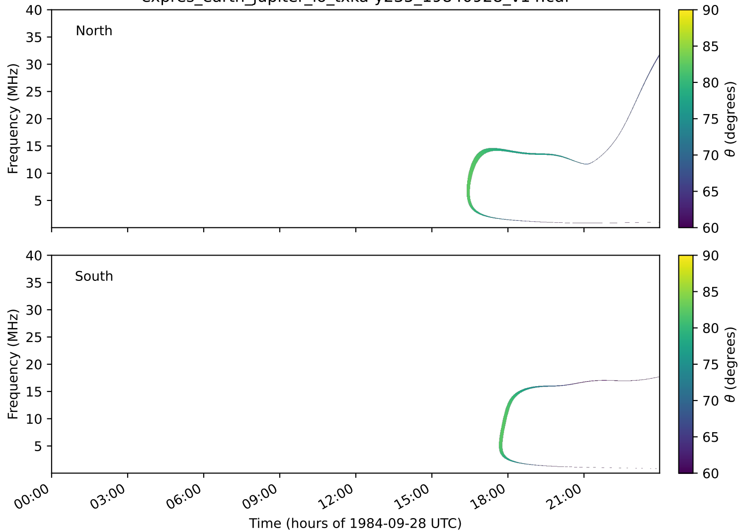
expres_earth_jupiter_io_txka-y235_19840928_v14.cdf
