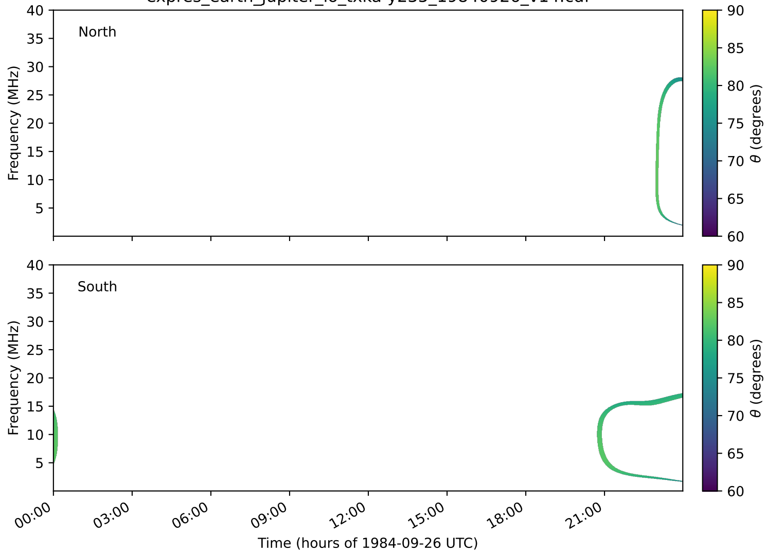
expres_earth_jupiter_io_txka-y235_19840926_v14.cdf
