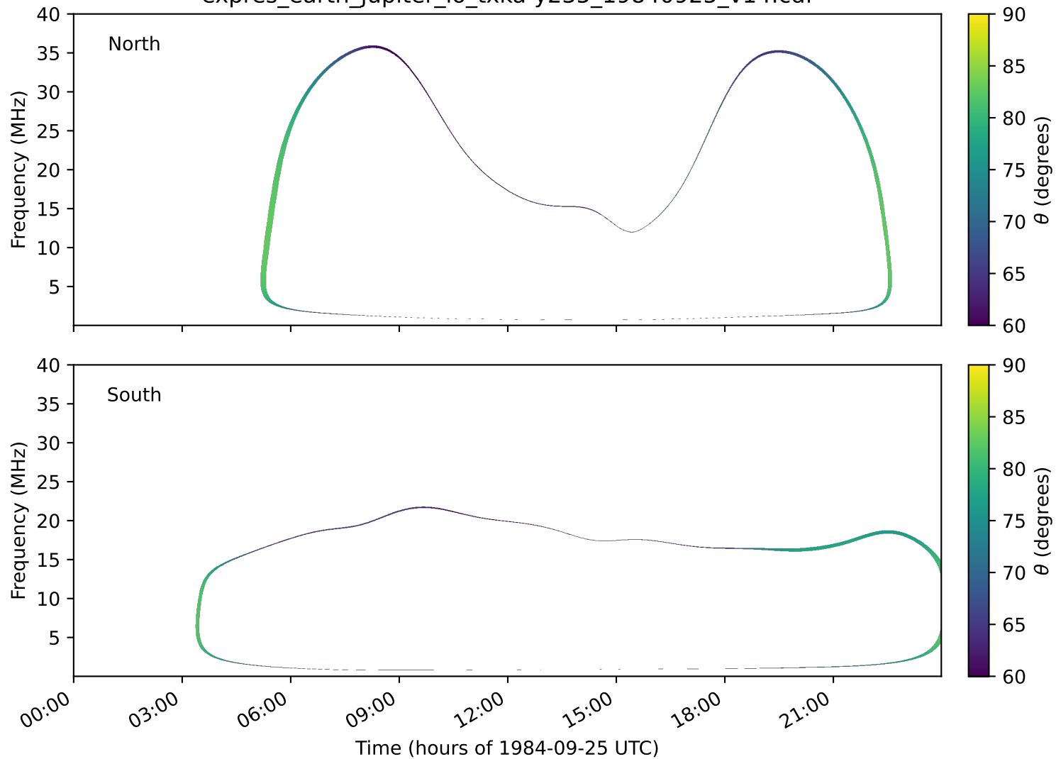
expres_earth_jupiter_io_txka-y235_19840925_v14.cdf
