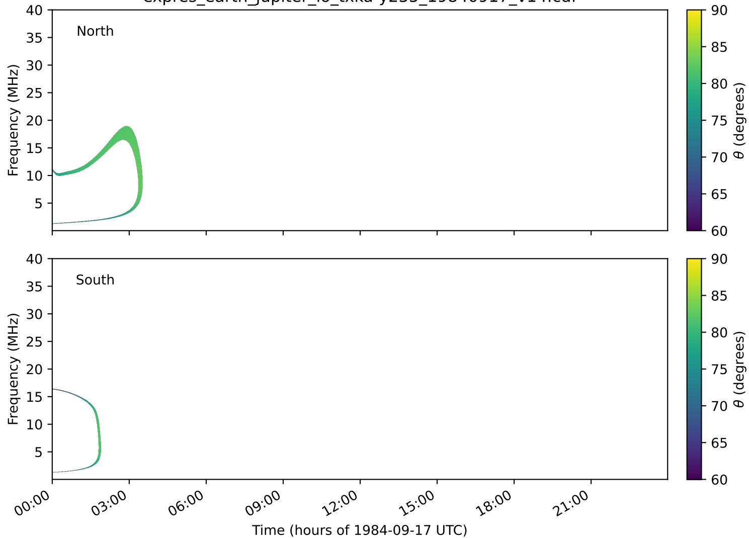
expres_earth_jupiter_io_txka-y235_19840917_v14.cdf
