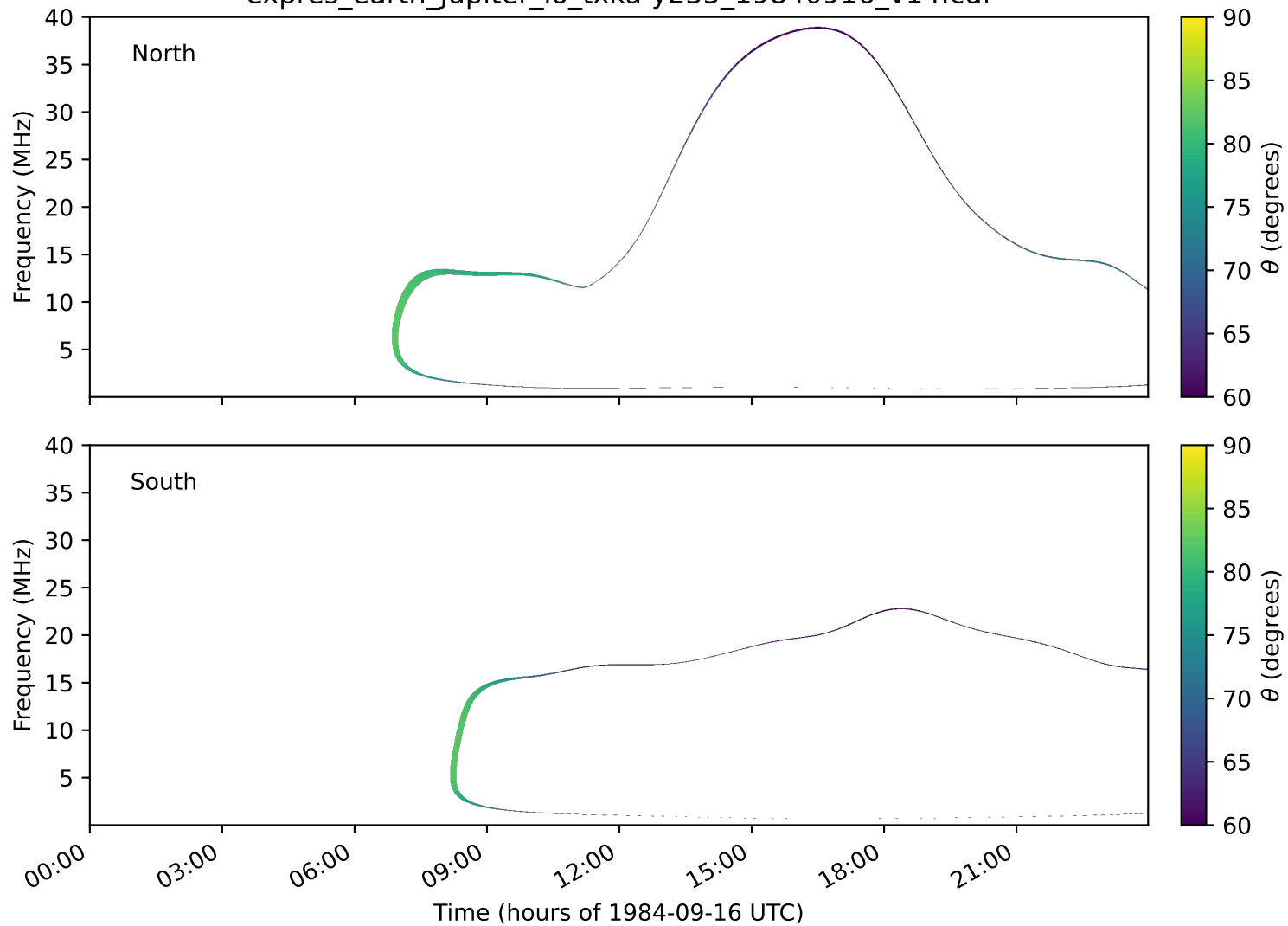
expres_earth_jupiter_io_txka-y235_19840916_v14.cdf
