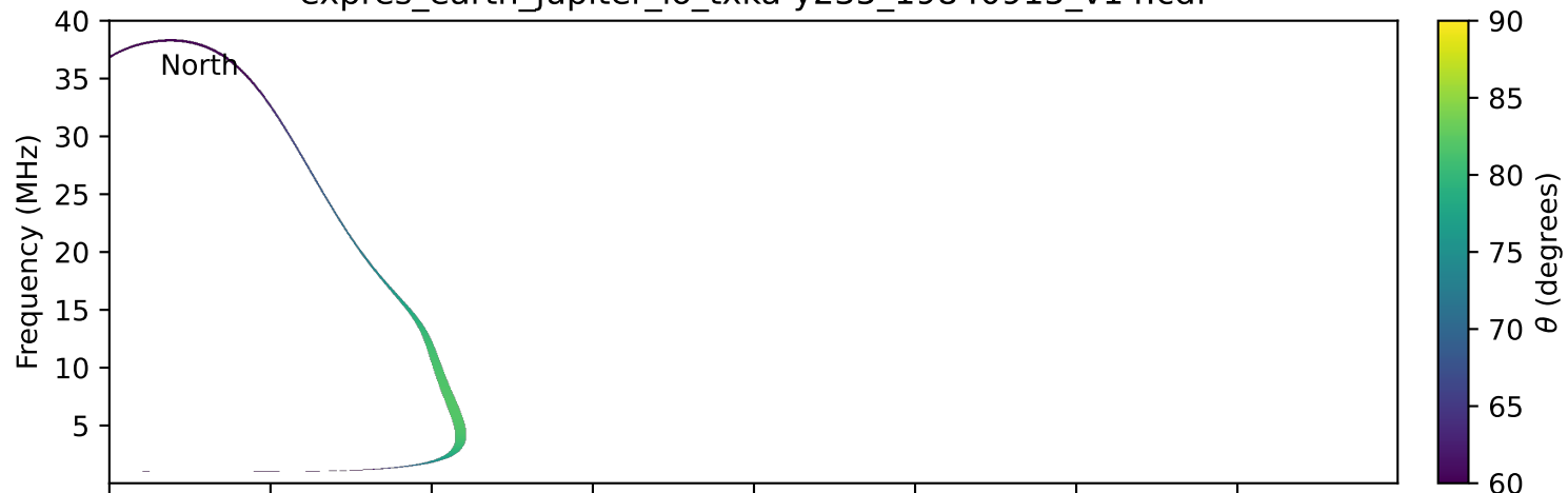
expres_earth_jupiter_io_txka-y235_19840915_v14.cdf
