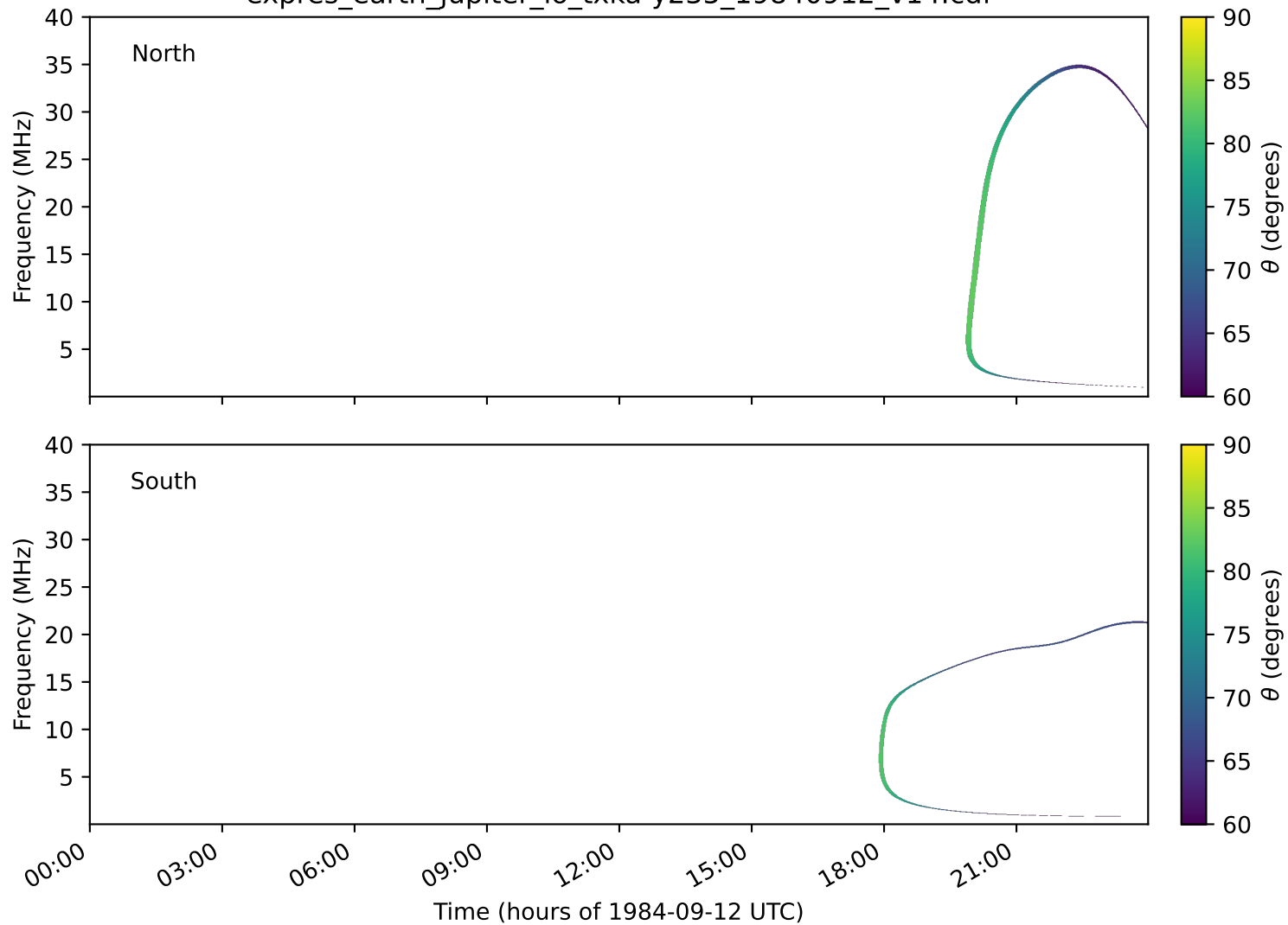
expres_earth_jupiter_io_txka-y235_19840912_v14.cdf
