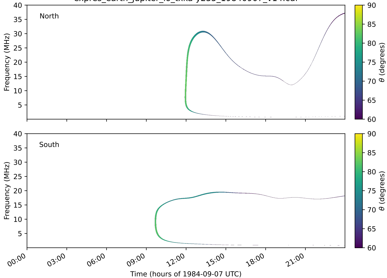
expres_earth_jupiter_io_txka-y235_19840907_v14.cdf
