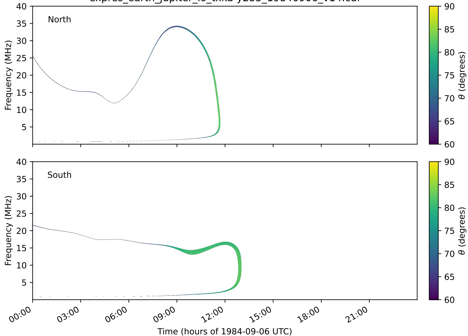
expres_earth_jupiter_io_txka-y235_19840906_v14.cdf
