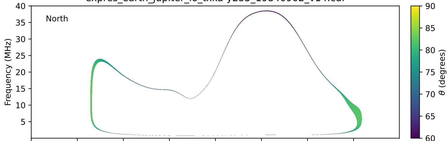
expres_earth_jupiter_io_txka-y235_19840902_v14.cdf
