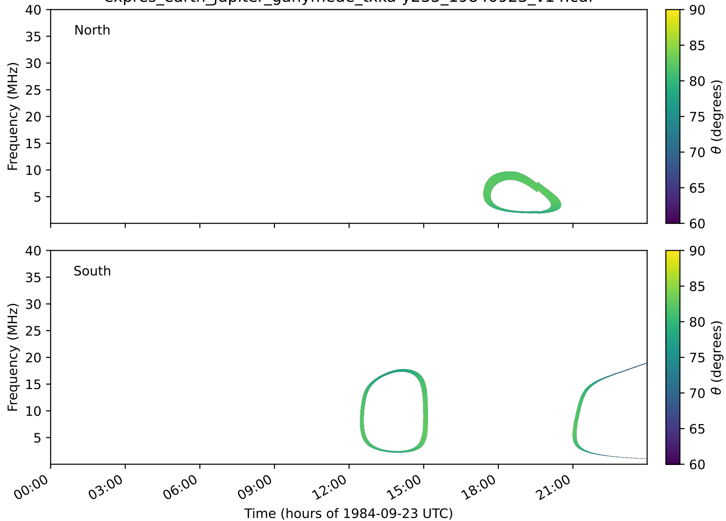
expres_earth_jupiter_ganymede_txka-y235_19840923_v14.cdf
