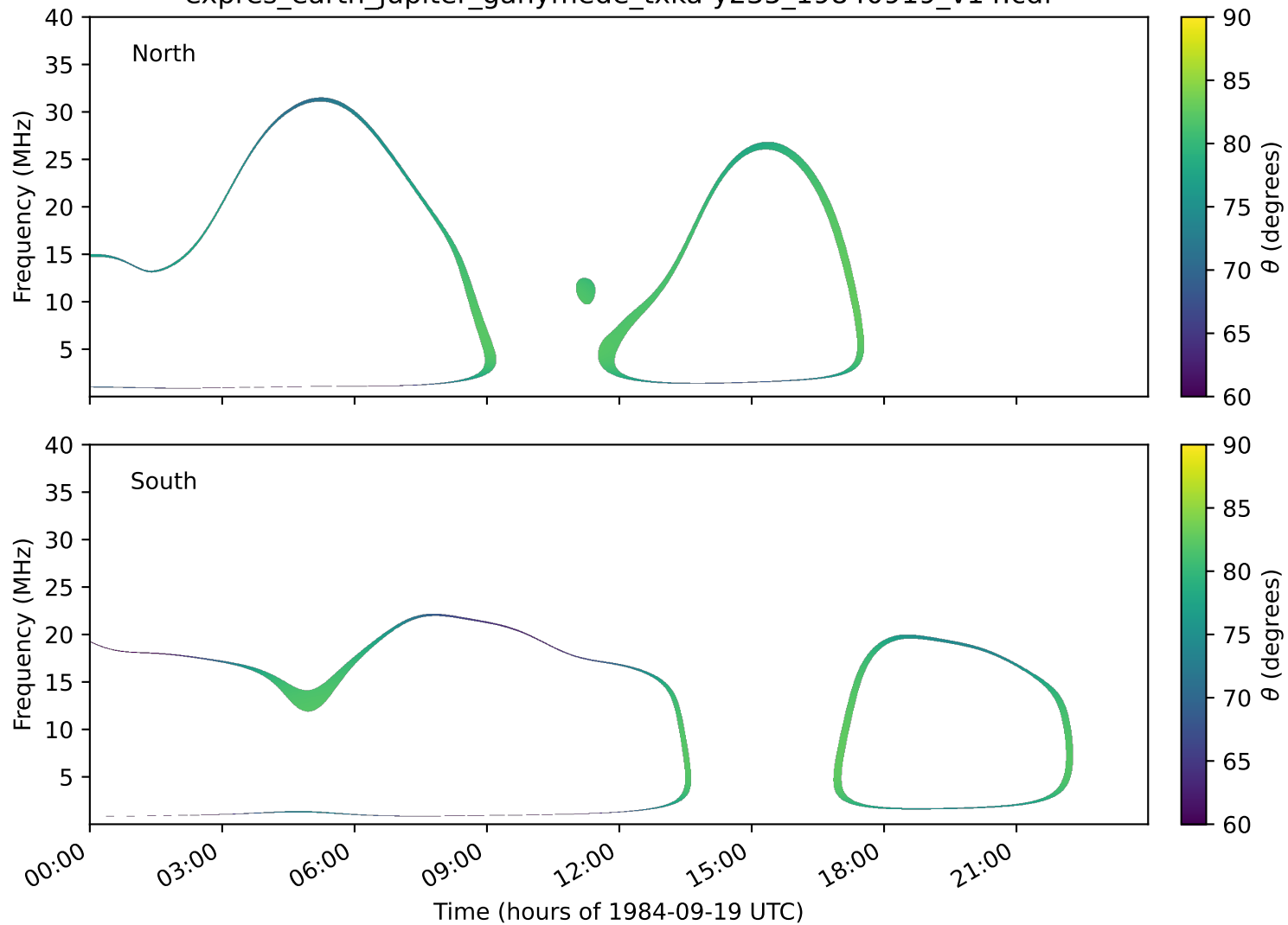
expres_earth_jupiter_ganymede_txka-y235_19840919_v14.cdf
