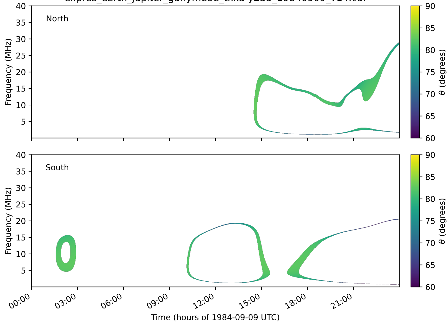
expres_earth_jupiter_ganymede_txka-y235_19840909_v14.cdf
