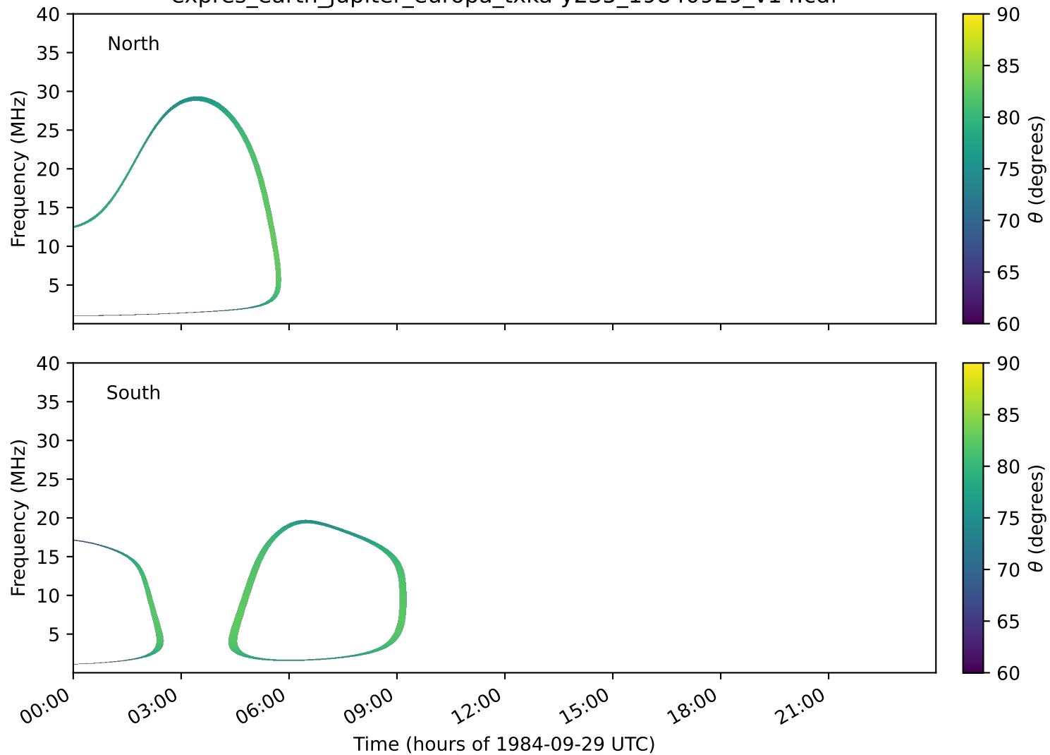
expres_earth_jupiter_europa_txka-y235_19840929_v14.cdf
