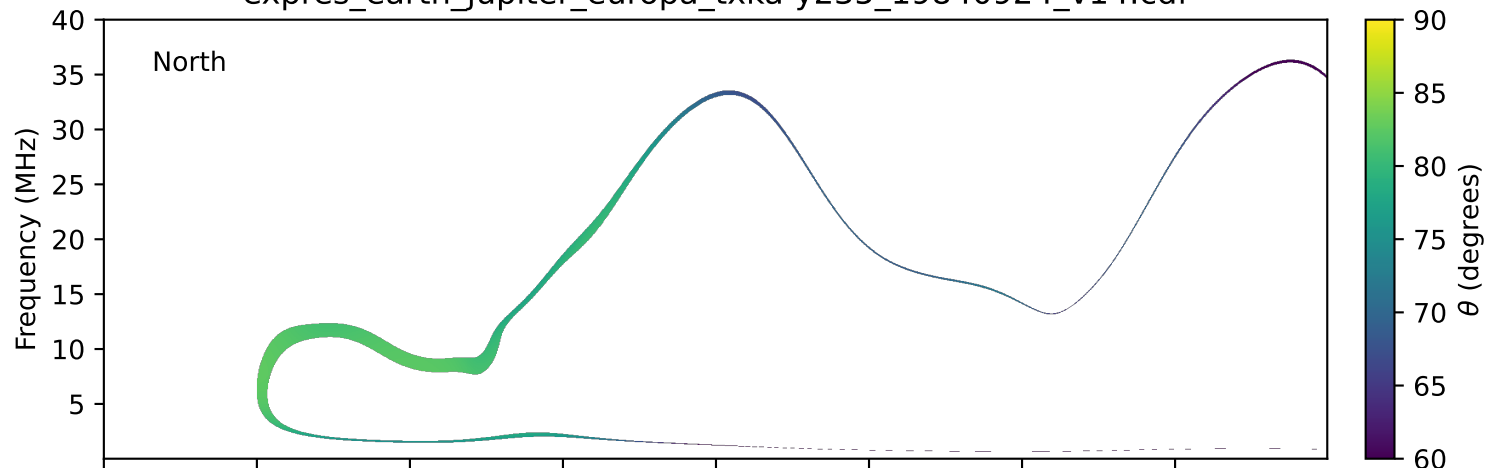
expres_earth_jupiter_europa_txka-y235_19840924_v14.cdf
