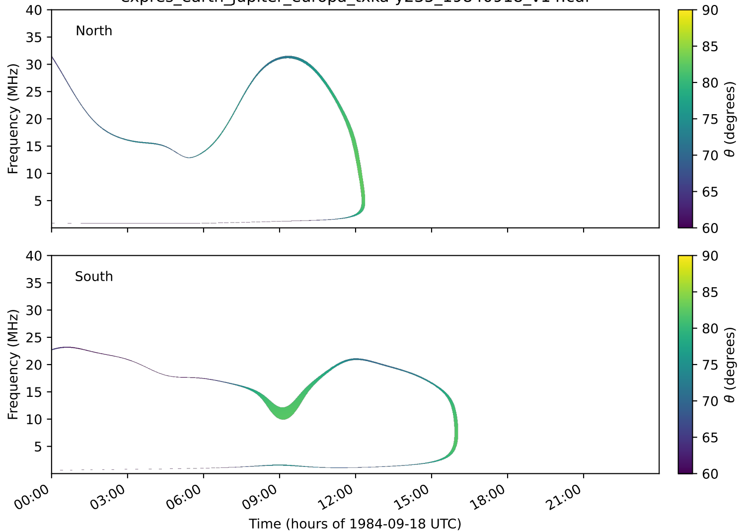
expres_earth_jupiter_europa_txka-y235_19840918_v14.cdf
