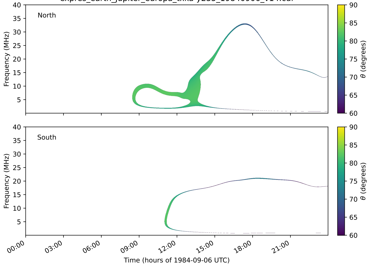
expres_earth_jupiter_europa_txka-y235_19840906_v14.cdf
