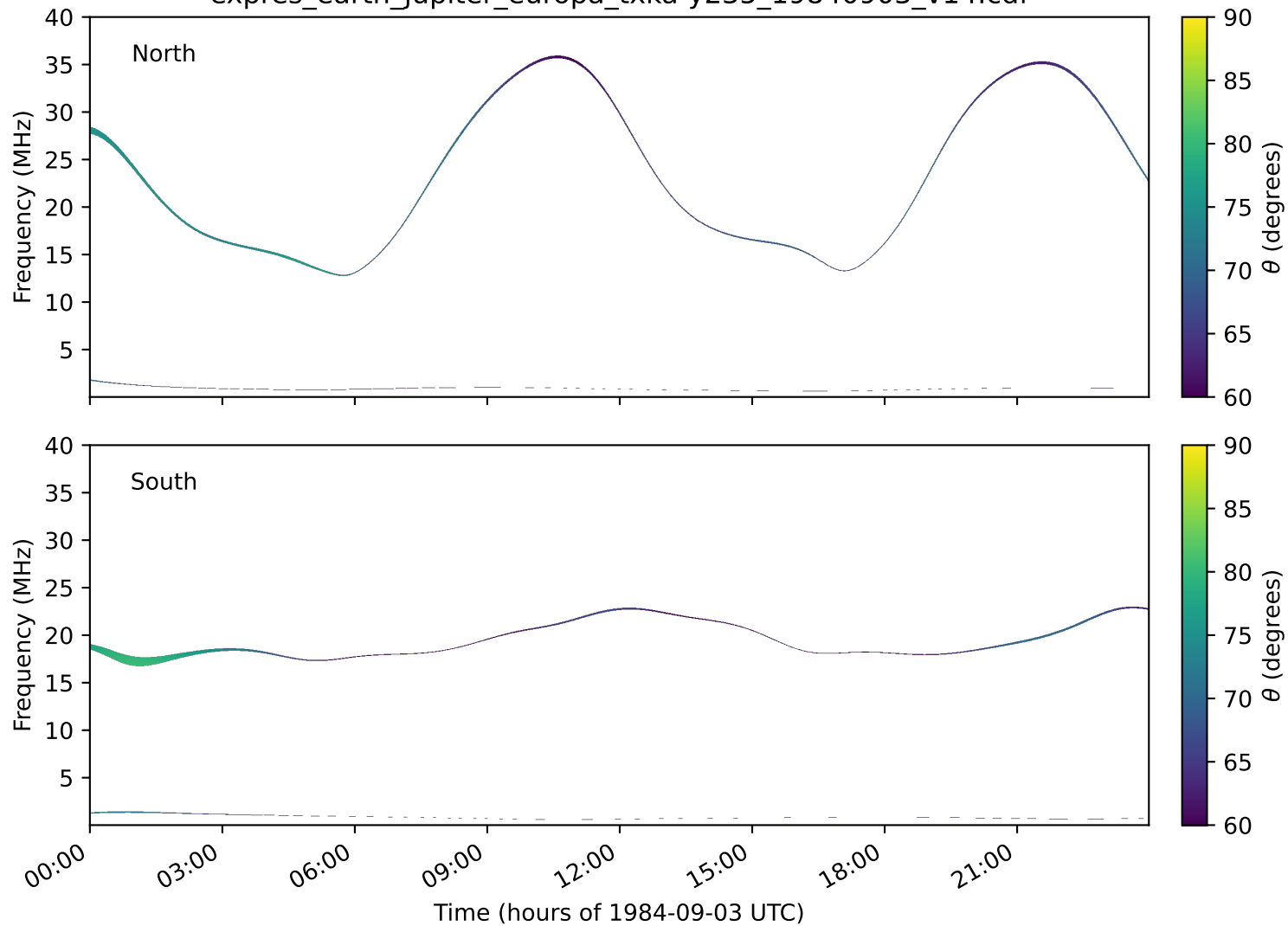
expres_earth_jupiter_europa_txka-y235_19840903_v14.cdf
