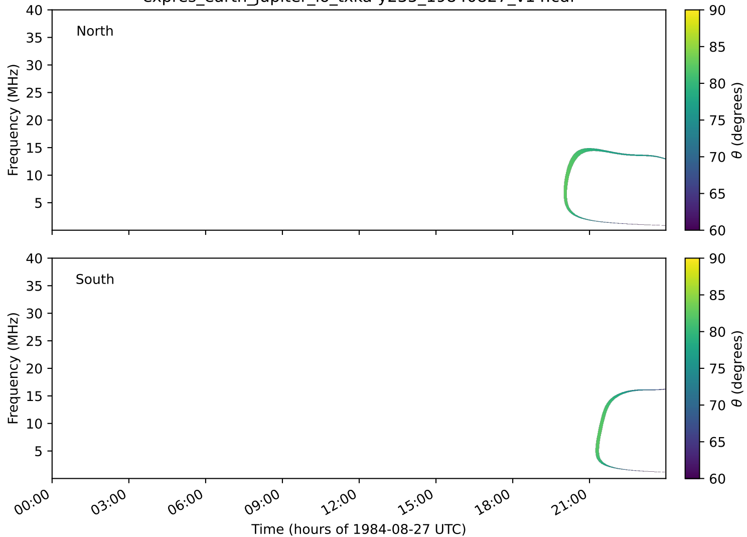
expres_earth_jupiter_io_txka-y235_19840827_v14.cdf
