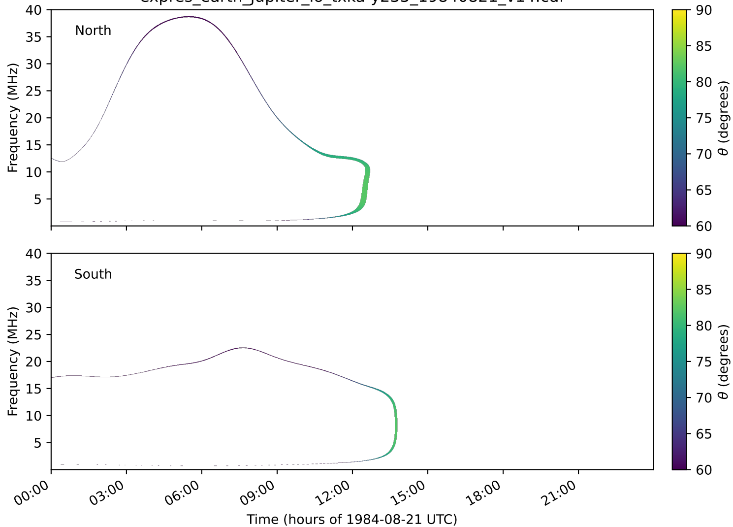
expres_earth_jupiter_io_txka-y235_19840821_v14.cdf
