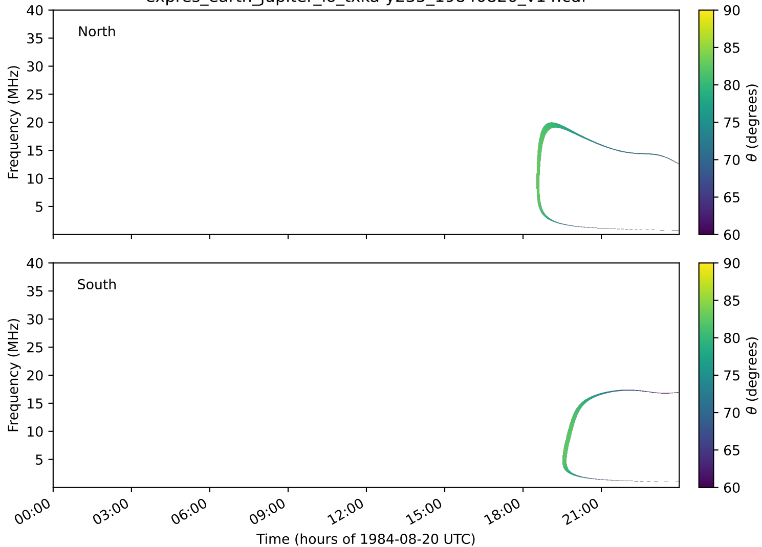
expres_earth_jupiter_io_txka-y235_19840820_v14.cdf
