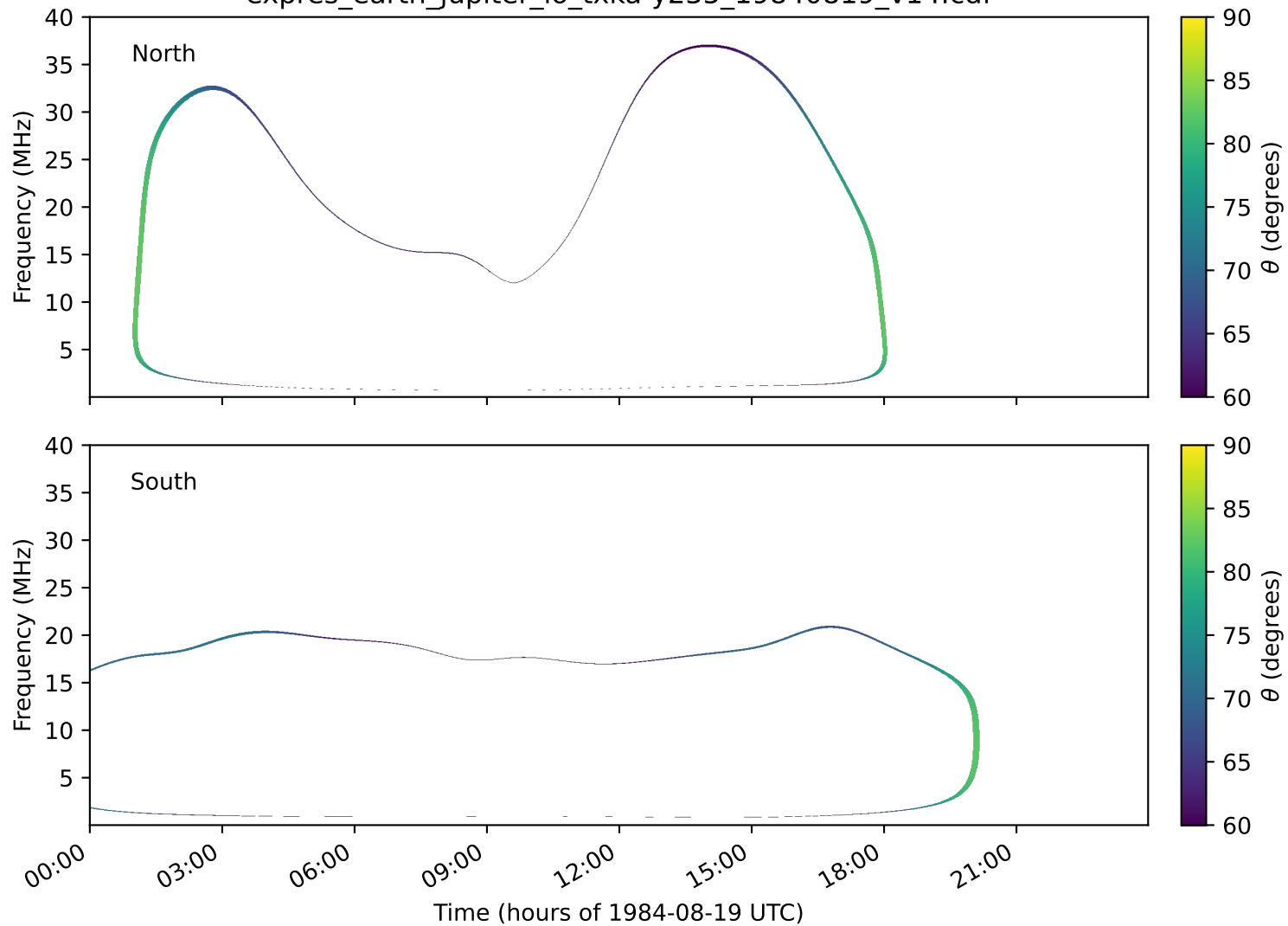
expres_earth_jupiter_io_txka-y235_19840819_v14.cdf
