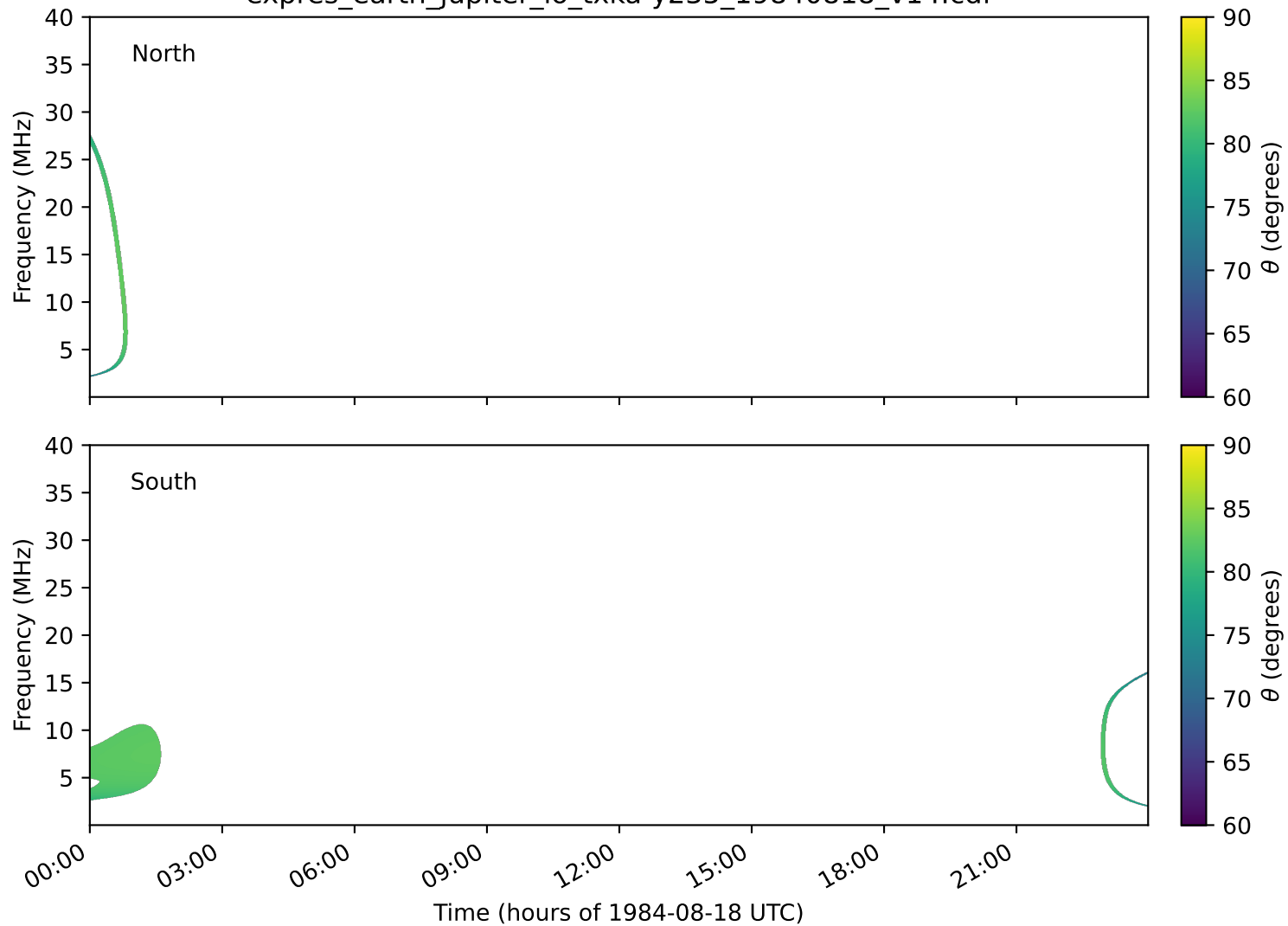
expres_earth_jupiter_io_txka-y235_19840818_v14.cdf
