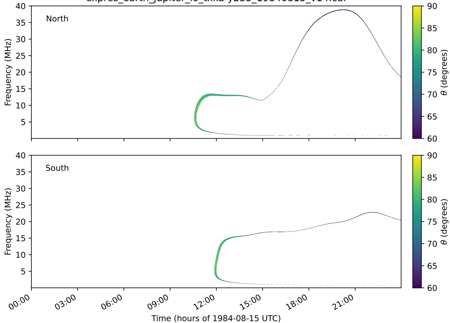
expres_earth_jupiter_io_txka-y235_19840815_v14.cdf
