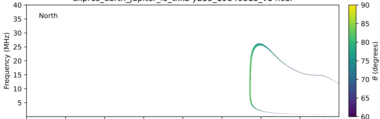
expres_earth_jupiter_io_txka-y235_19840813_v14.cdf
