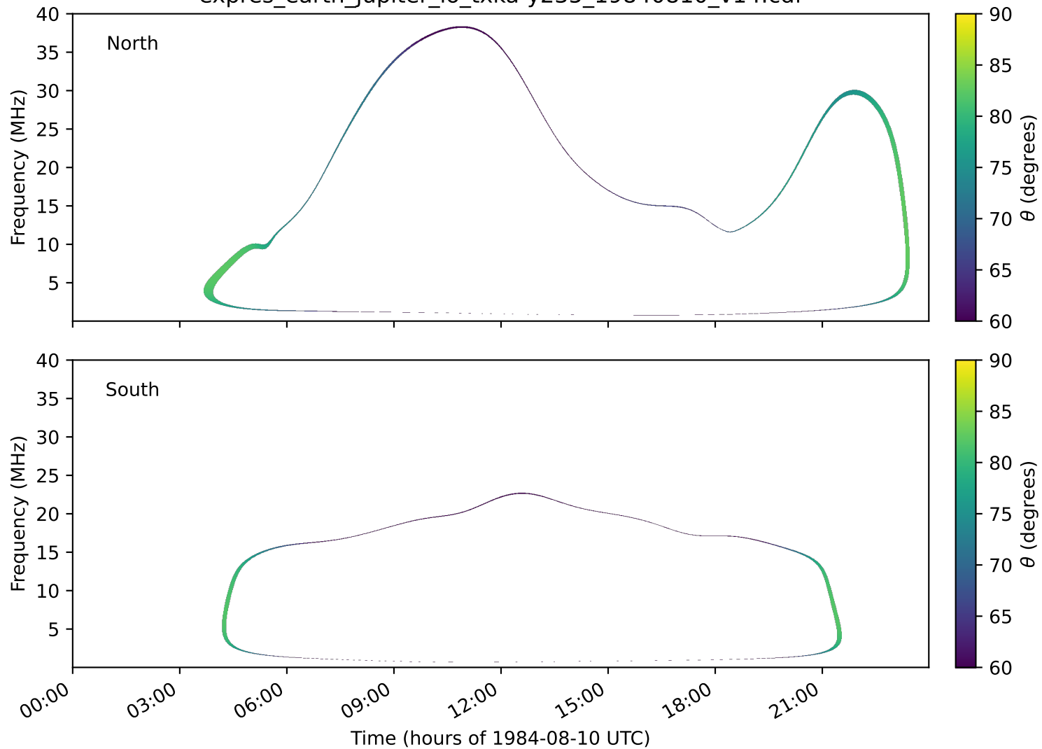
expres_earth_jupiter_io_txka-y235_19840810_v14.cdf
