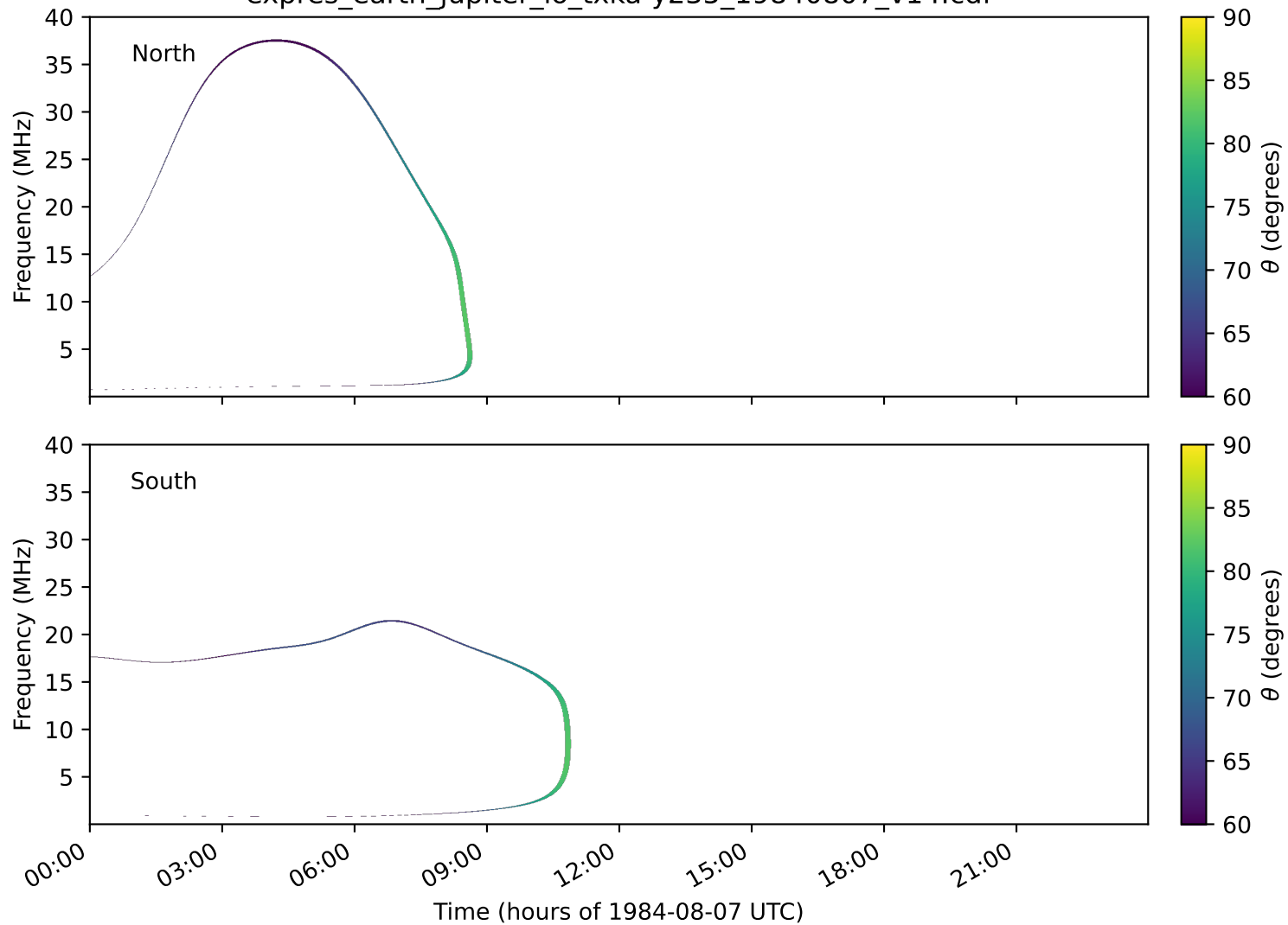
expres_earth_jupiter_io_txka-y235_19840807_v14.cdf
