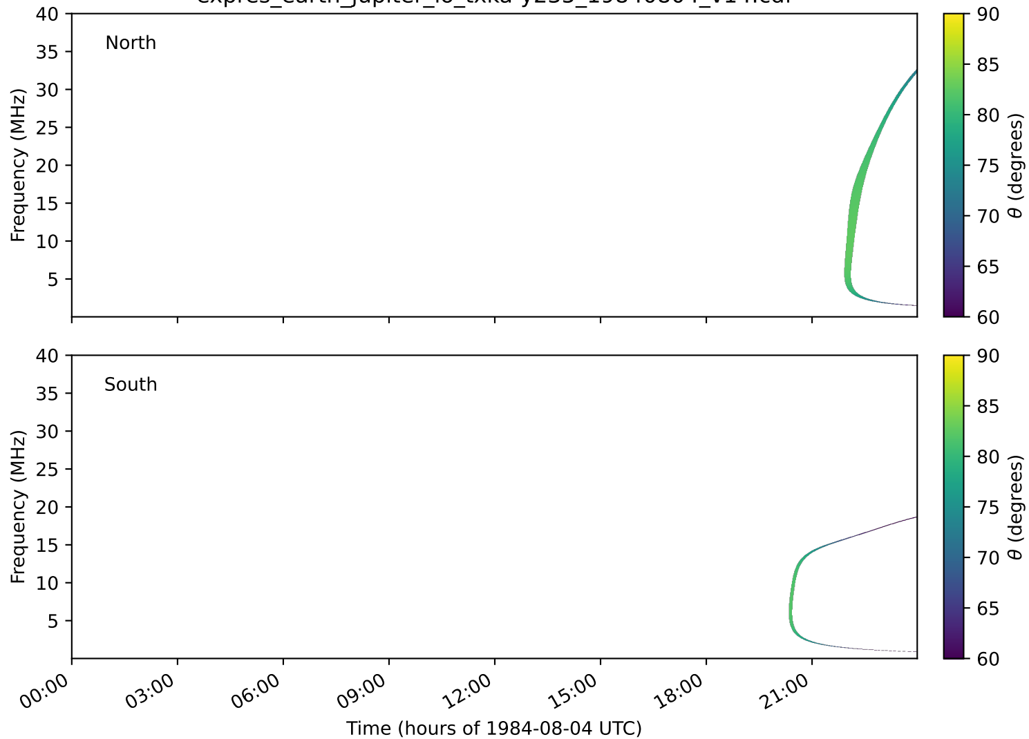
expres_earth_jupiter_io_txka-y235_19840804_v14.cdf
