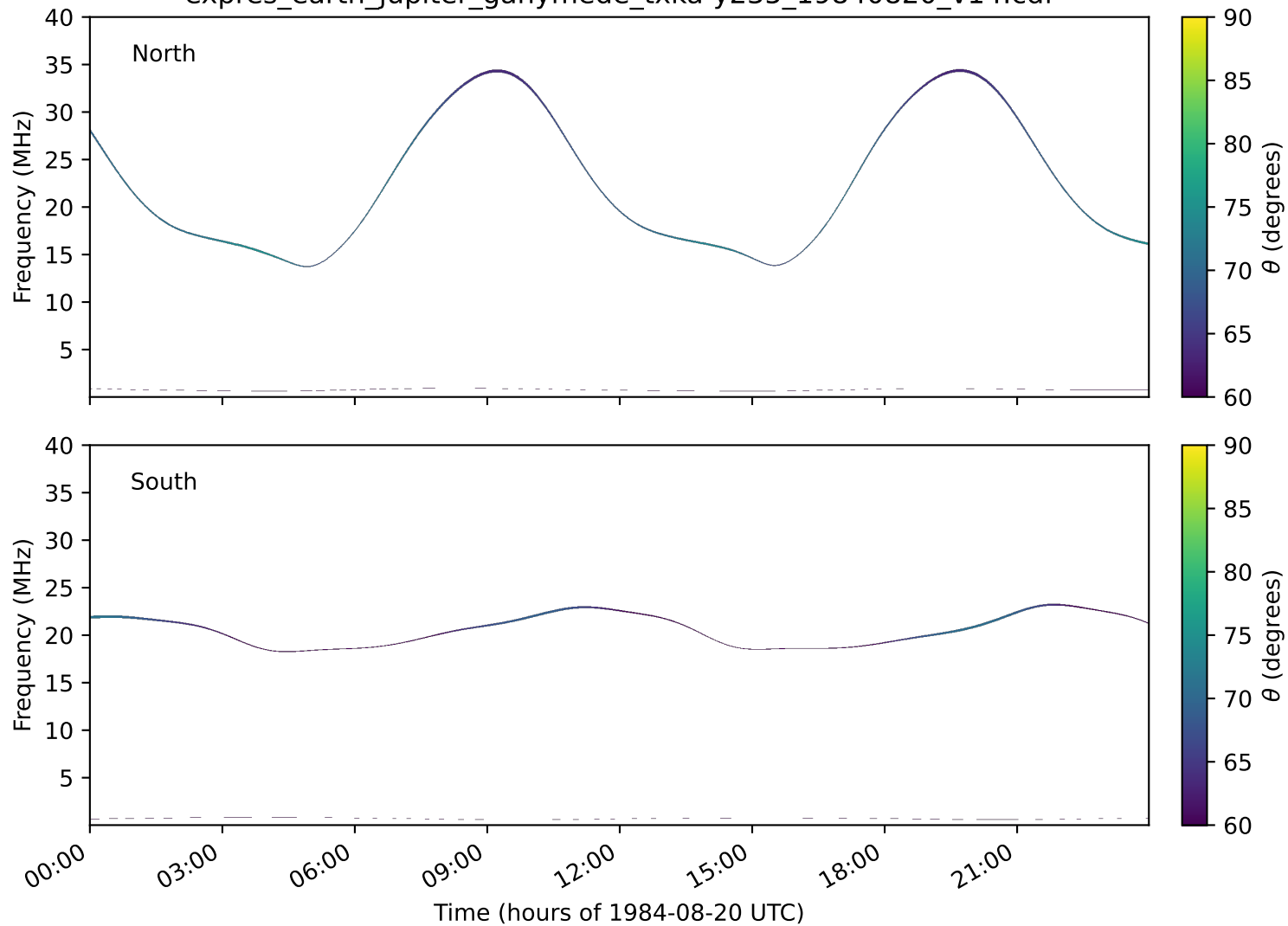
expres_earth_jupiter_ganymede_txka-y235_19840820_v14.cdf
