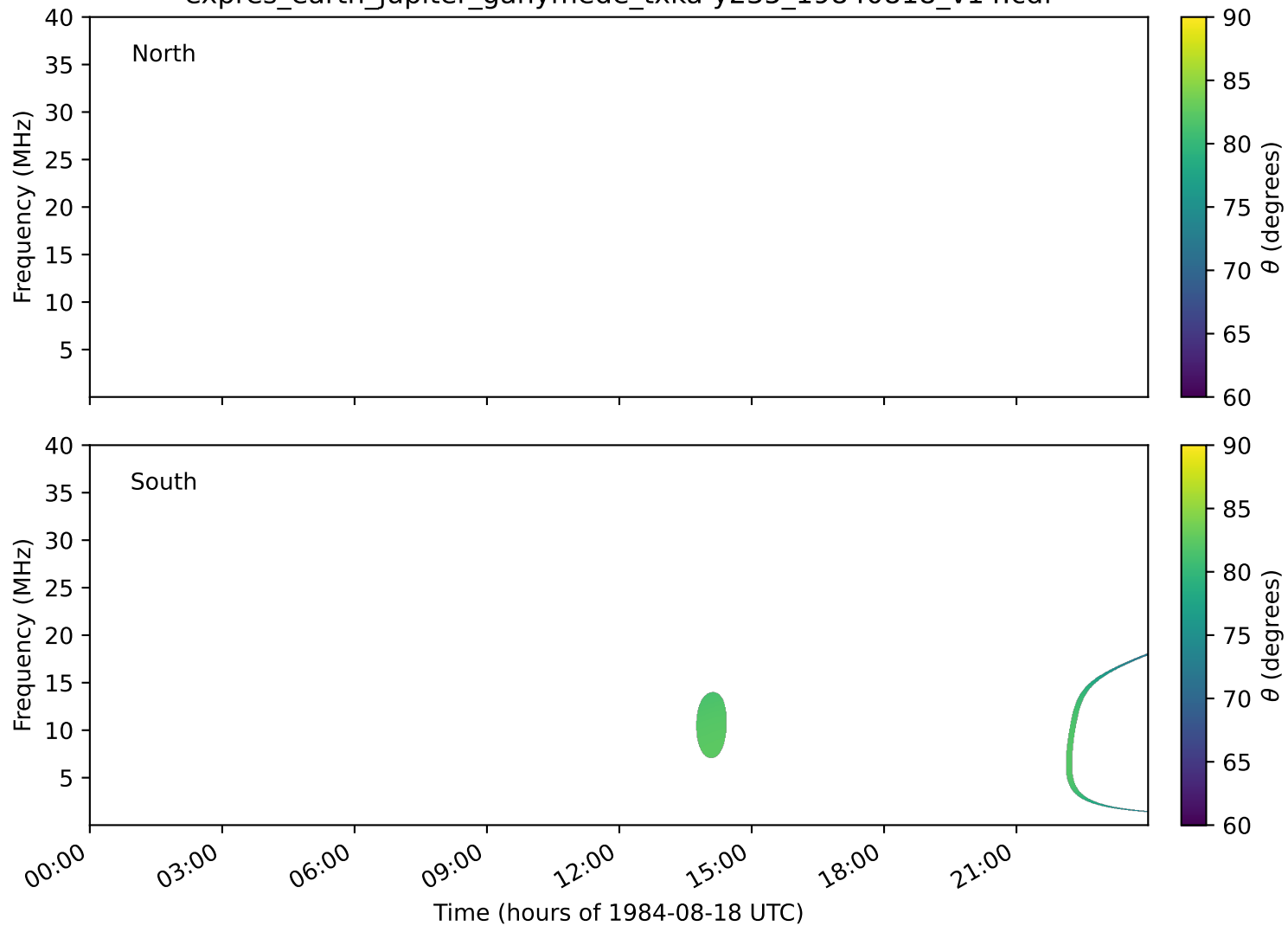
expres_earth_jupiter_ganymede_txka-y235_19840818_v14.cdf
