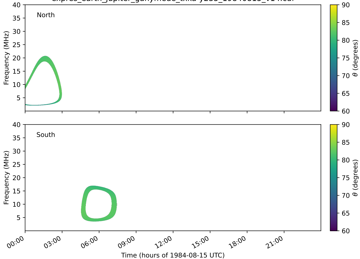
expres_earth_jupiter_ganymede_txka-y235_19840815_v14.cdf
