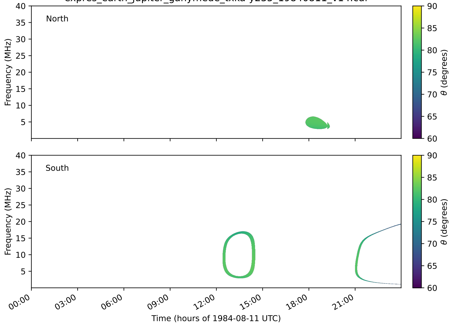
expres_earth_jupiter_ganymede_txka-y235_19840811_v14.cdf
