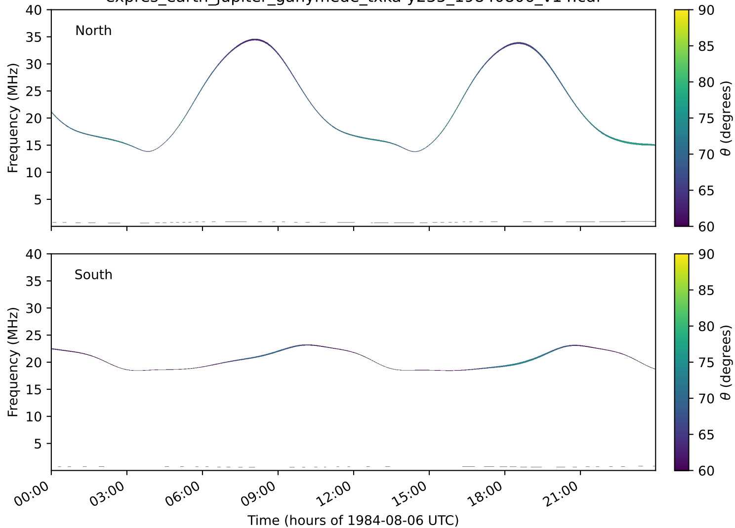
expres_earth_jupiter_ganymede_txka-y235_19840806_v14.cdf
