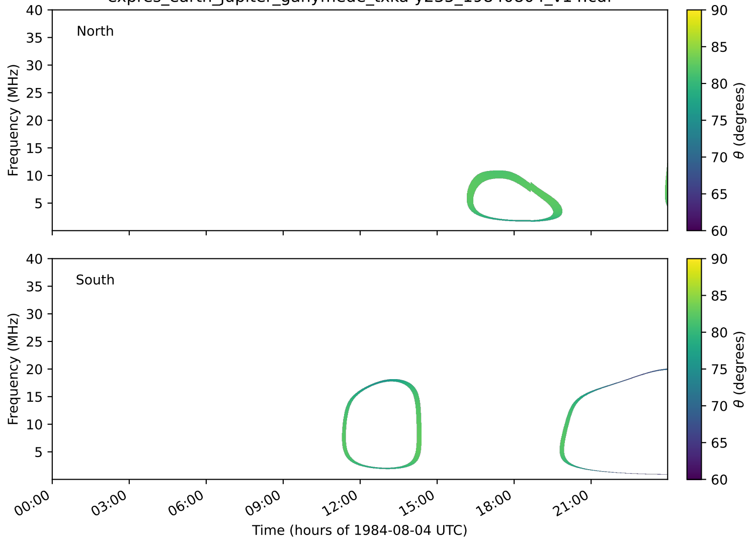
expres_earth_jupiter_ganymede_txka-y235_19840804_v14.cdf
