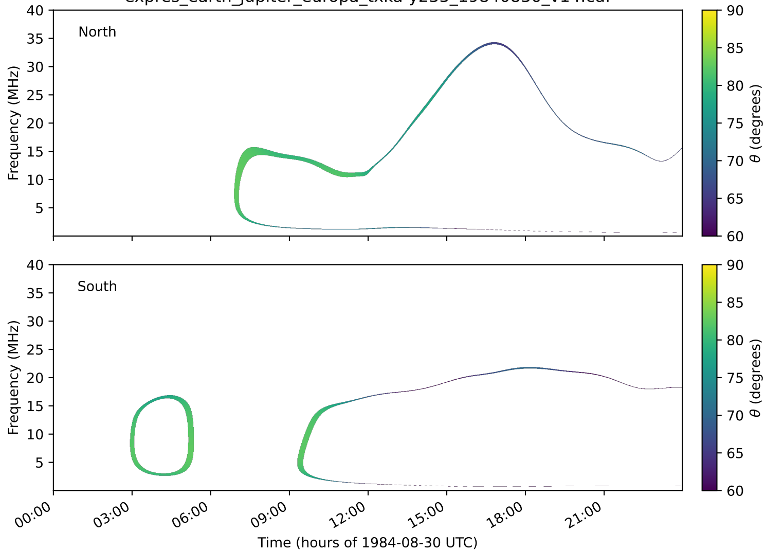
expres_earth_jupiter_europa_txka-y235_19840830_v14.cdf
