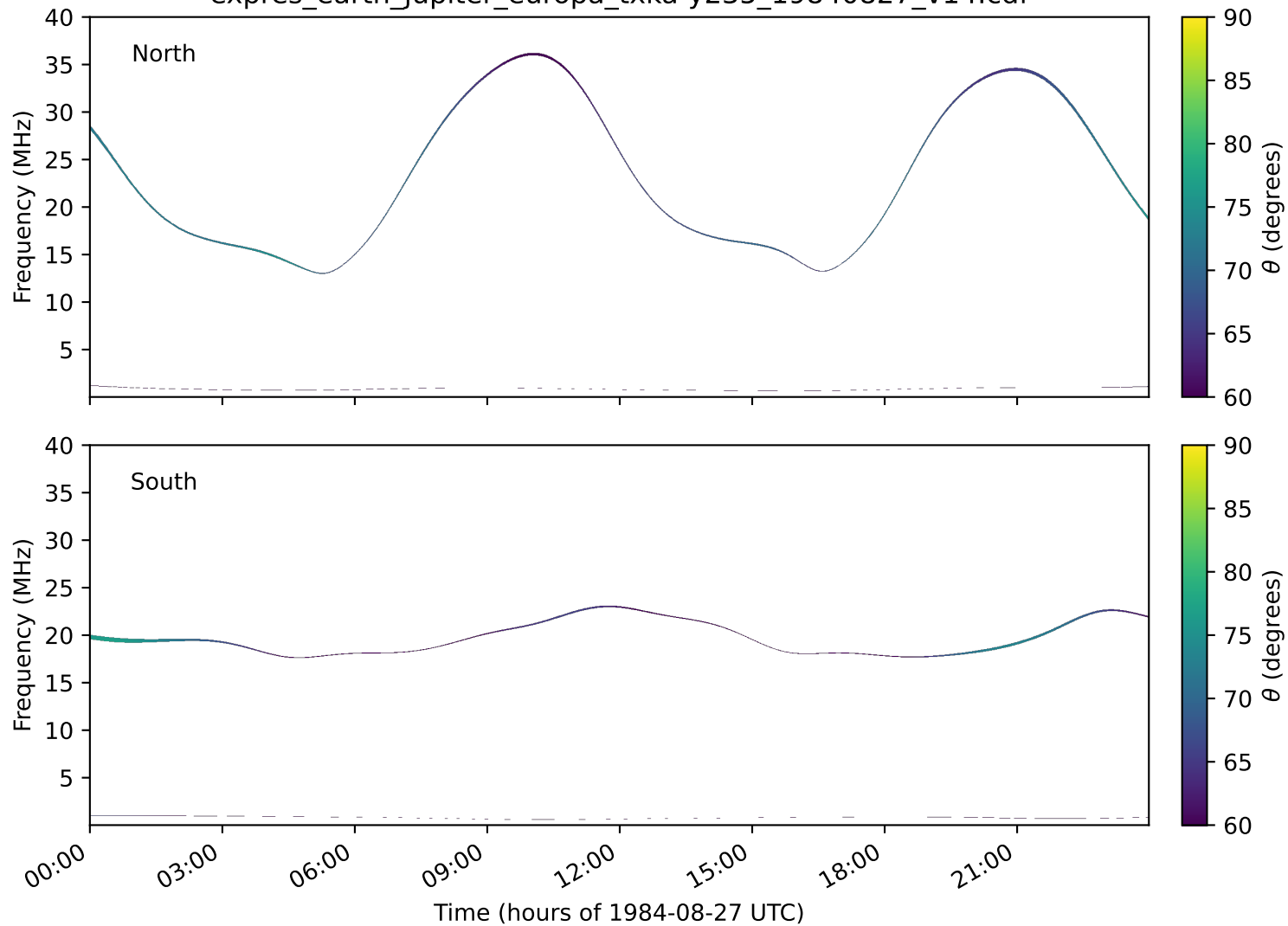
expres_earth_jupiter_europa_txka-y235_19840827_v14.cdf
