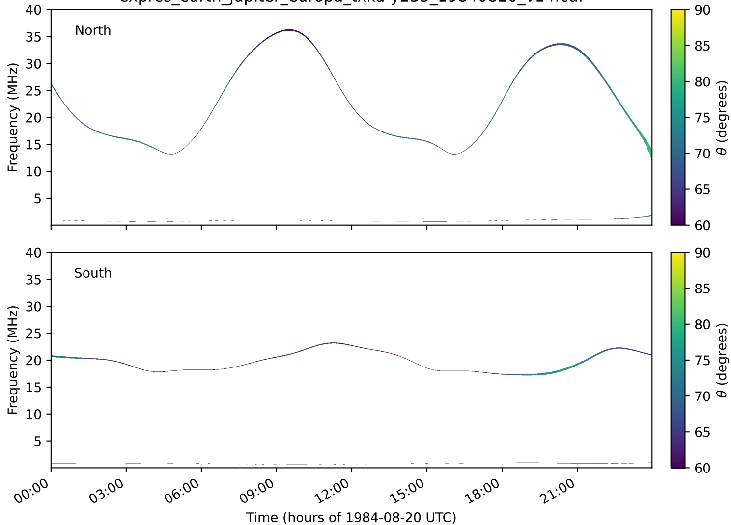
expres_earth_jupiter_europa_txka-y235_19840820_v14.cdf
