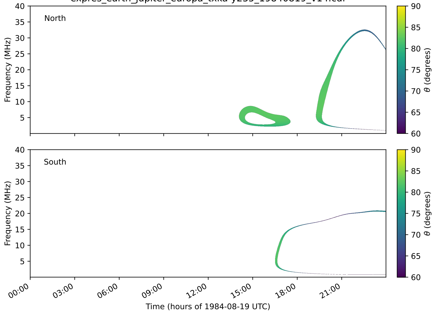
expres_earth_jupiter_europa_txka-y235_19840819_v14.cdf
